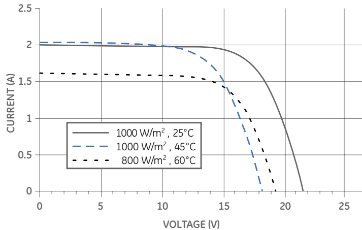
Typical I-V Curve for GEPV-030 Module
